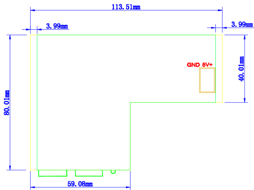
Fig. 2 CVT310 internal dimensions
